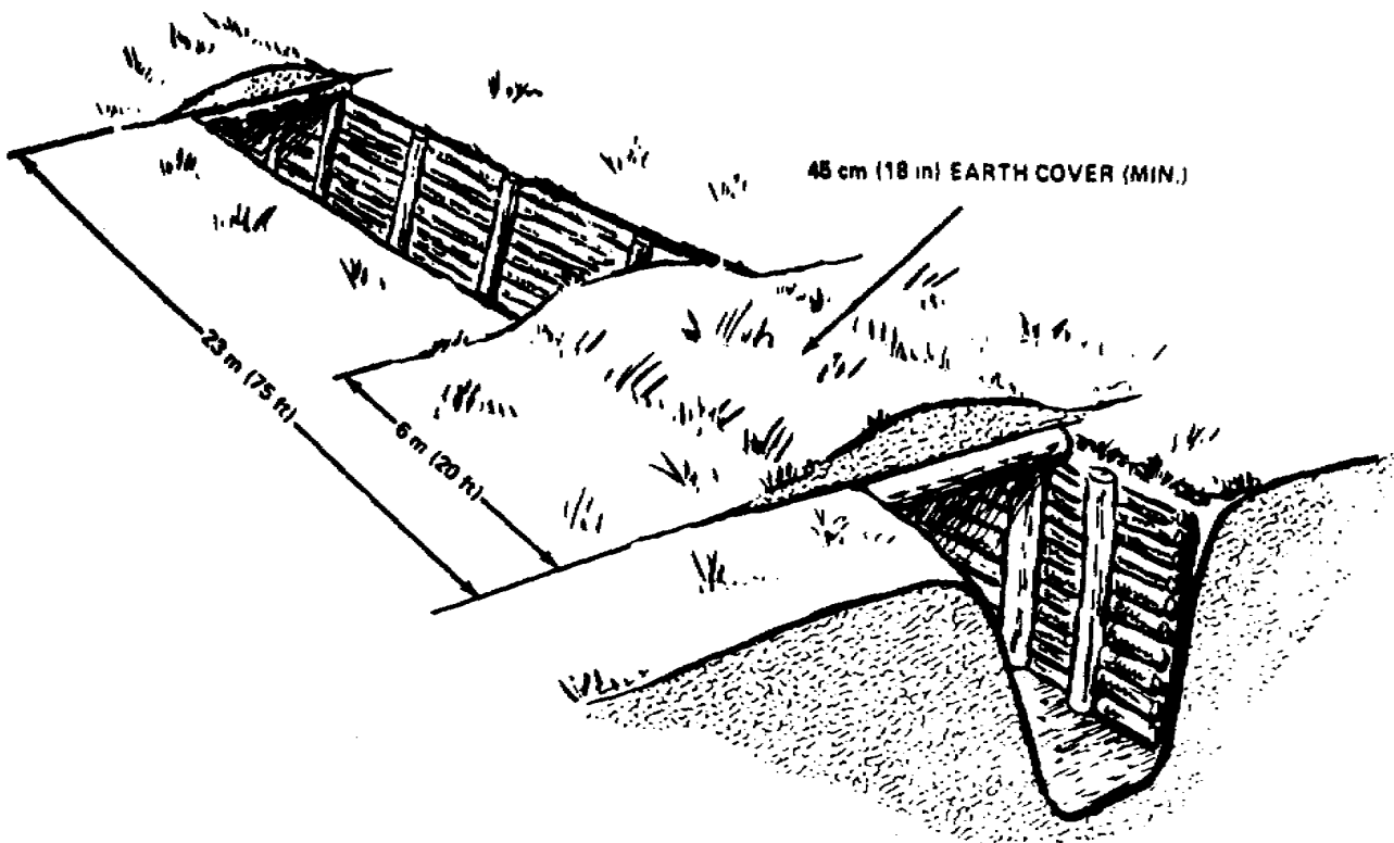
Figure 2-11. Revetted fighting trench with cover.
